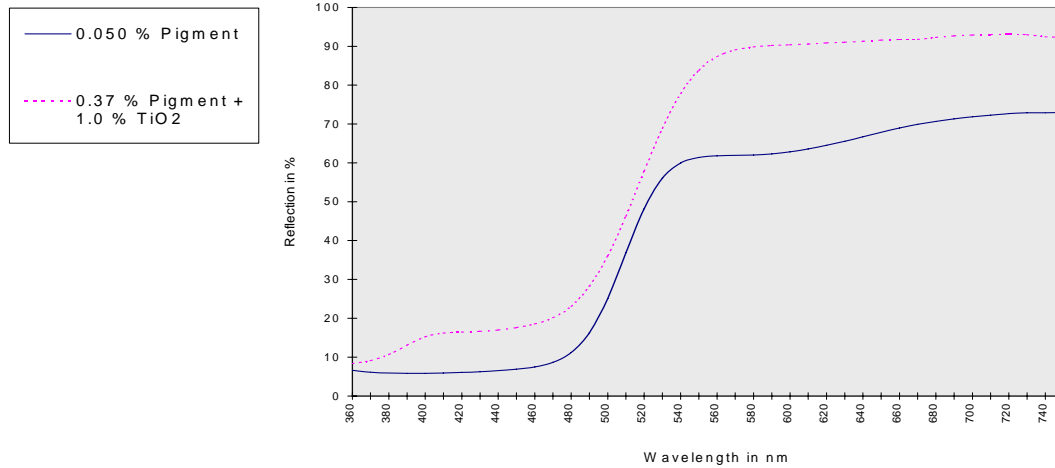
Reflection curve BAYPLAST Yellow G Gran in PP (2 mm thickness)
